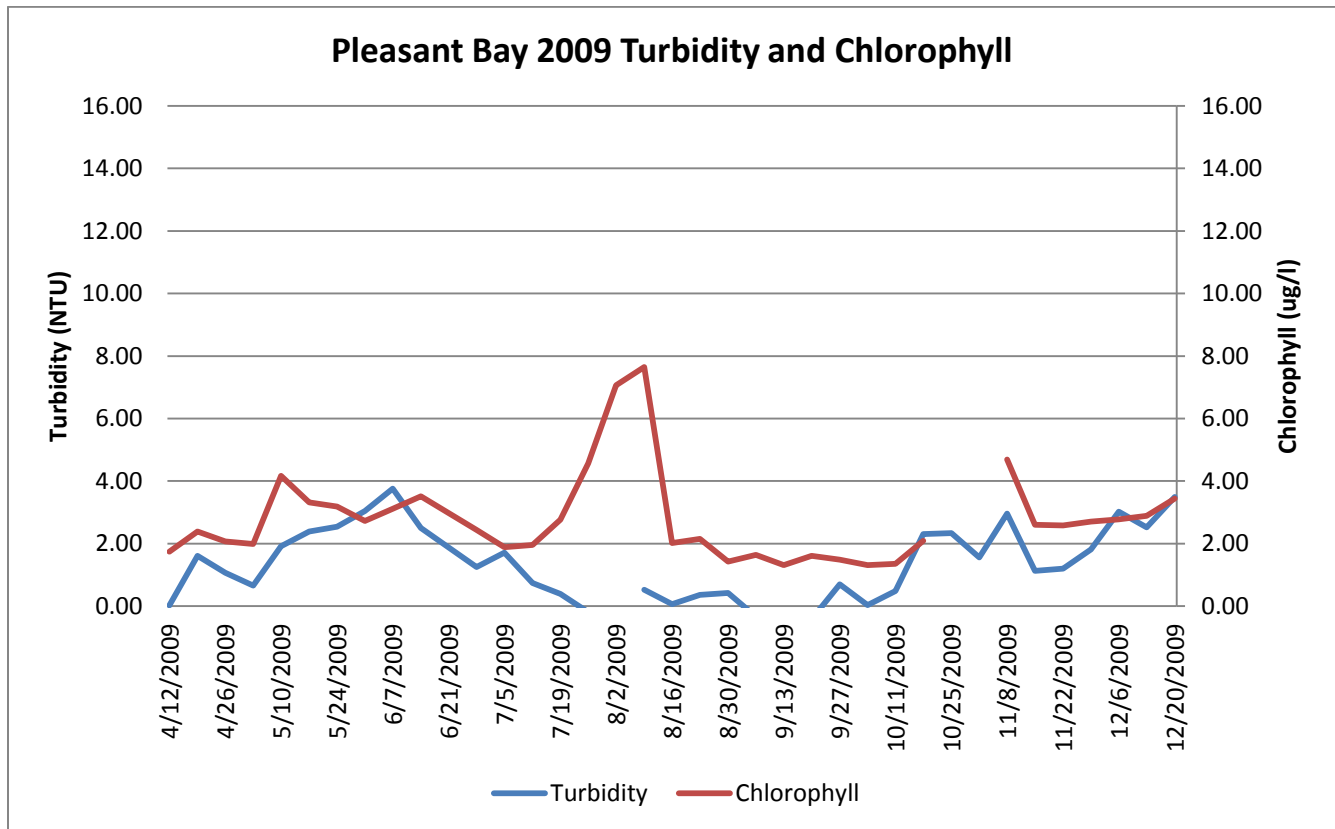
Weekly mean turbidity and chlorophyll as measured at Portanimicut Landing in Pleasant Bay during 2009.
