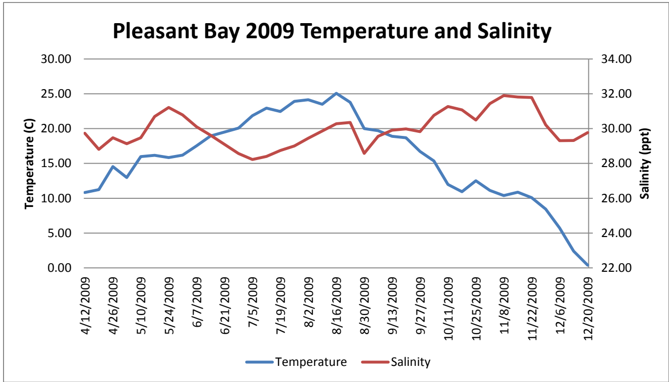
Weekly mean water temperature and salinity as measured at Portanimicut Landing in Pleasant Bay during 2009.
