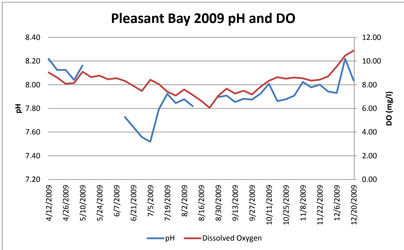
Weekly mean pH and dissolved oxygen as measured at Portanimicut Landing in Pleasant Bay during 2009.
