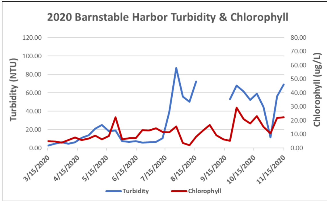
Weekly mean turbidity and chlorophyll as measured at Scudders Landing in Barnstable Harbor during 2020.
