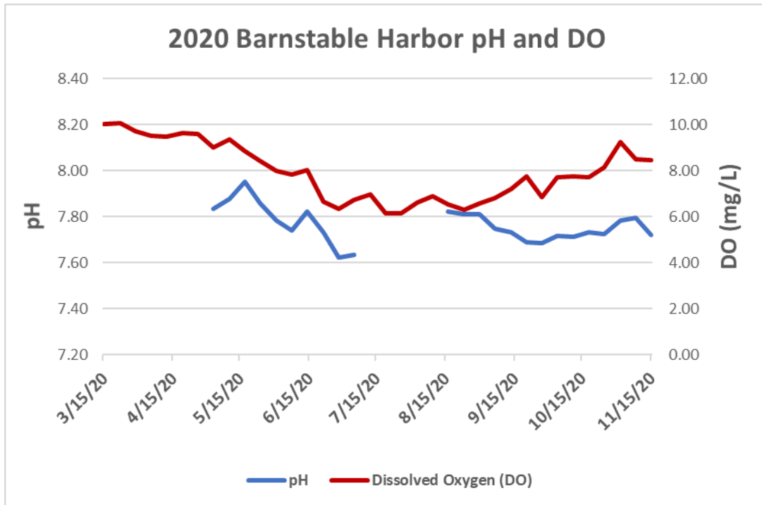
Weekly mean pH and dissolved oxygen as measured at Scudders Landing in Barnstable Harbor during 2020.
