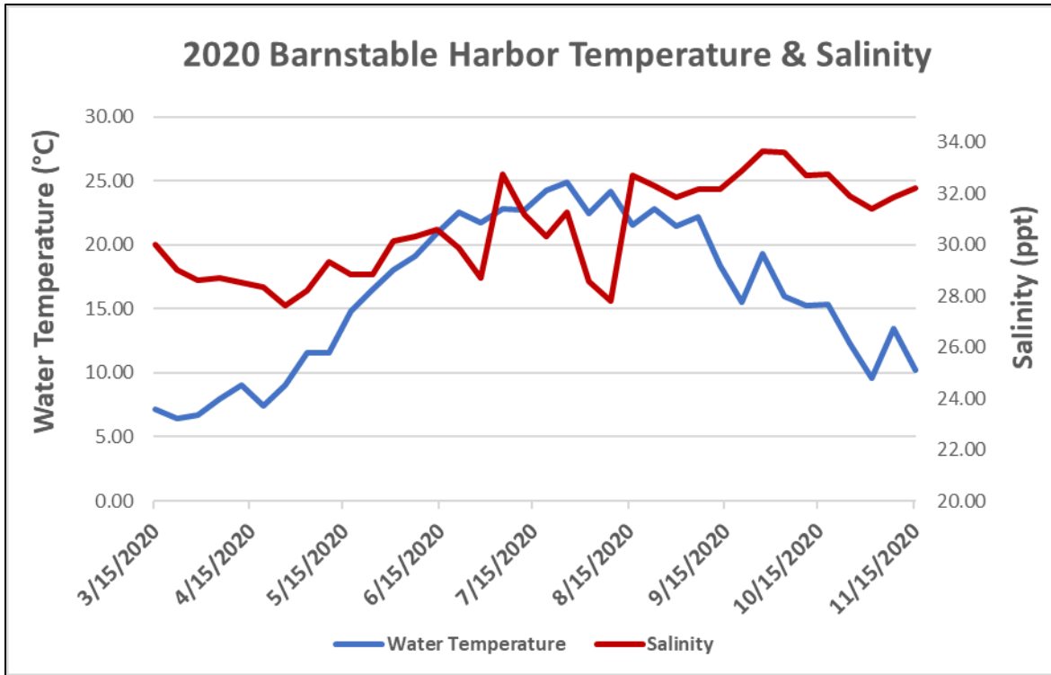
Weekly mean water temperature and salinity as measured at Scudders Landing in Barnstable Harbor during 2020.
