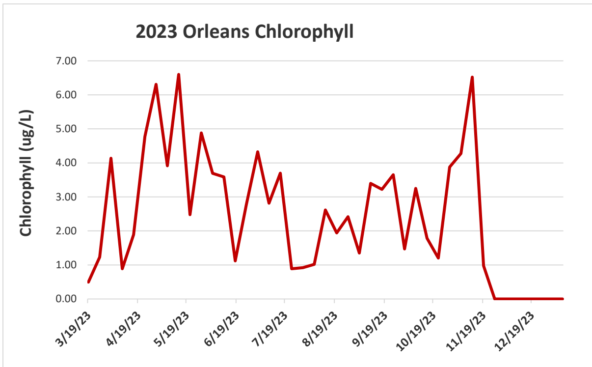
Weekly mean chlorophyll as measured in Orleans during 2023.
