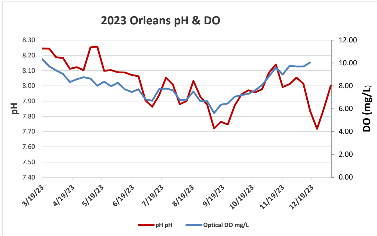
Weekly mean pH and dissolved oxygen as measured in Orleans during 2023.
