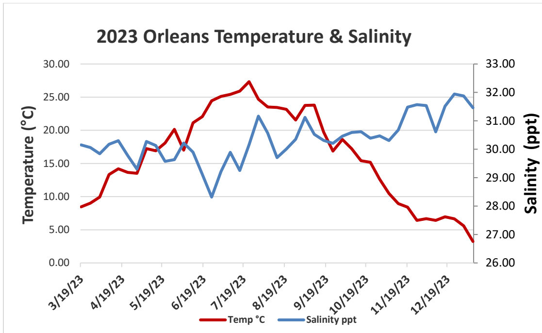
Weekly mean water temperature and salinity as measured in Orleans during 2023.
